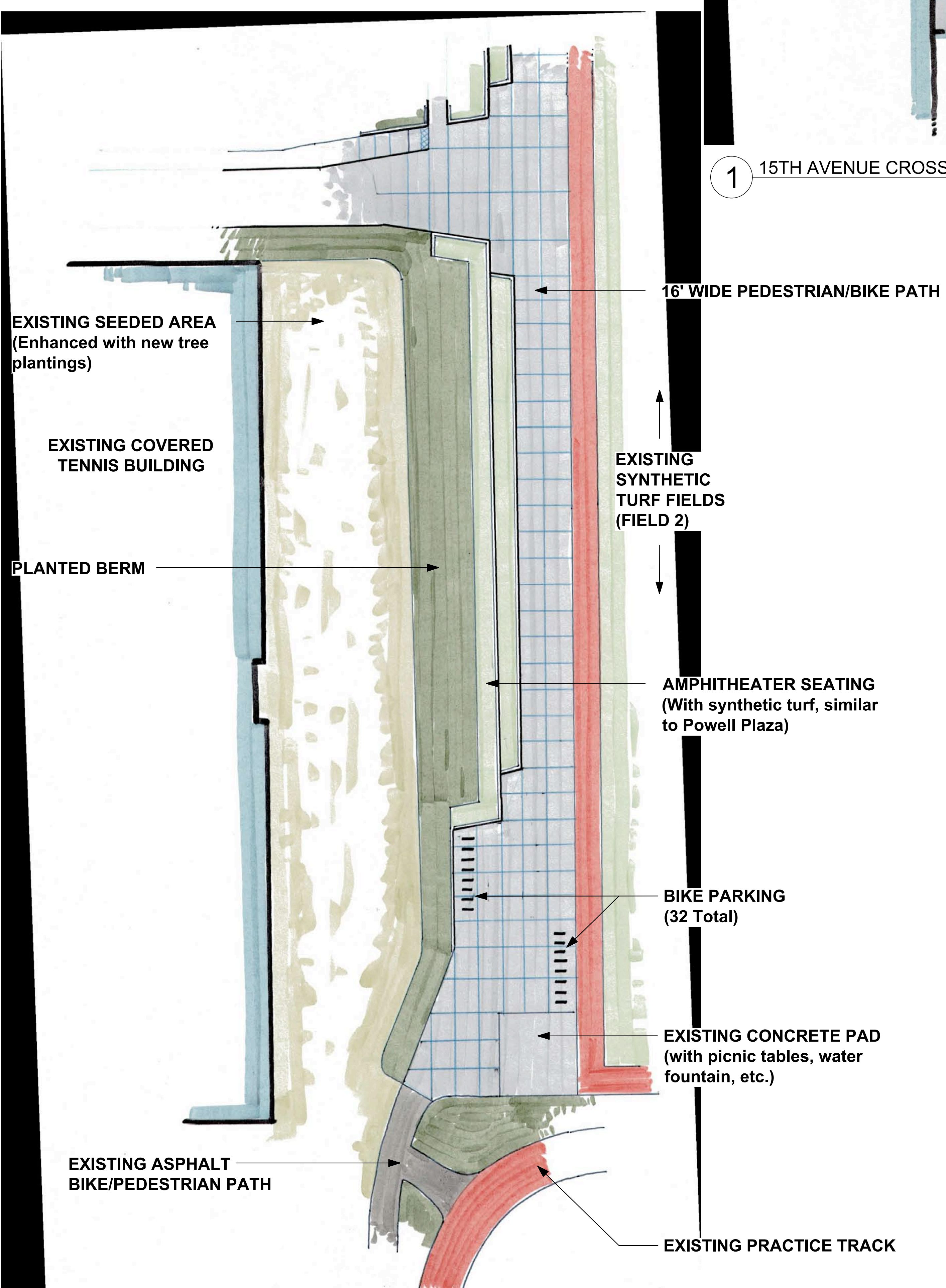
2 SOUTH BIKE/PEDESTRIAN PATH OPTION
