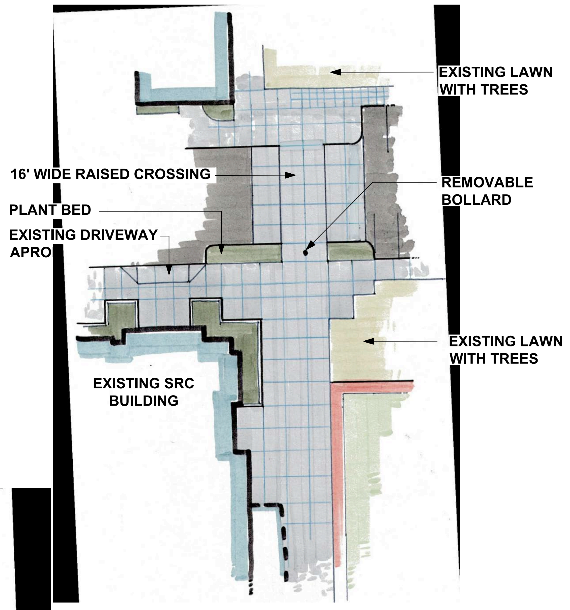
1 15TH AVENUE CROSSING OPTION
